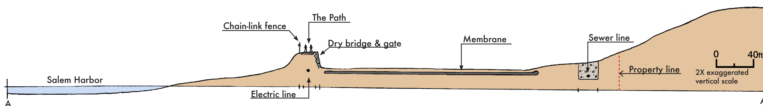
Marblehead's main electrical line runs under The Path and a sewer line runs along the southern property boundary.
