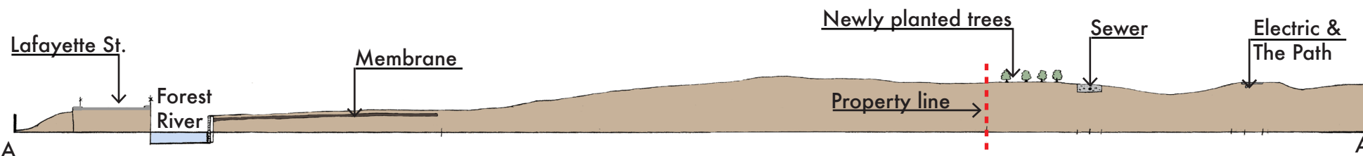
Section across the property shows the gentle slopes, the river wall without a barrier, and the Forest River at mid-tide.
